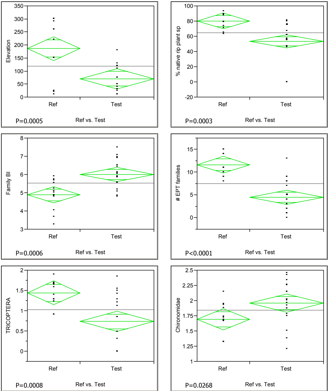
Figure 15 Reference Group vs. Test Group T-Tests, Sites in a Low-Moderate Elevation, Gradient, and Stream Order Classification
